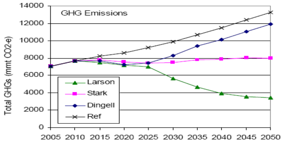
Figure 9. Emission trajectories.
